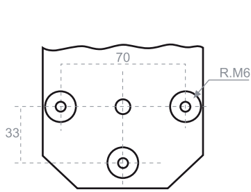
BCR1000 mounting
